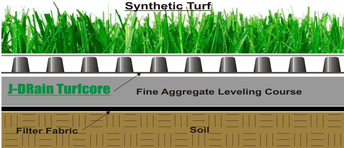
Fig 1. Turfcore Sections
